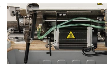
Stepping motor drive for the thread trimmer and auto-lifter
